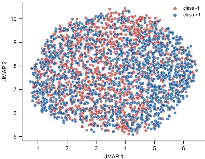
UMAP after PCA-50
