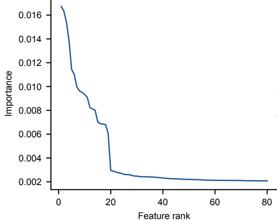
Random Forest
