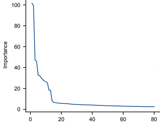
Random Forest
