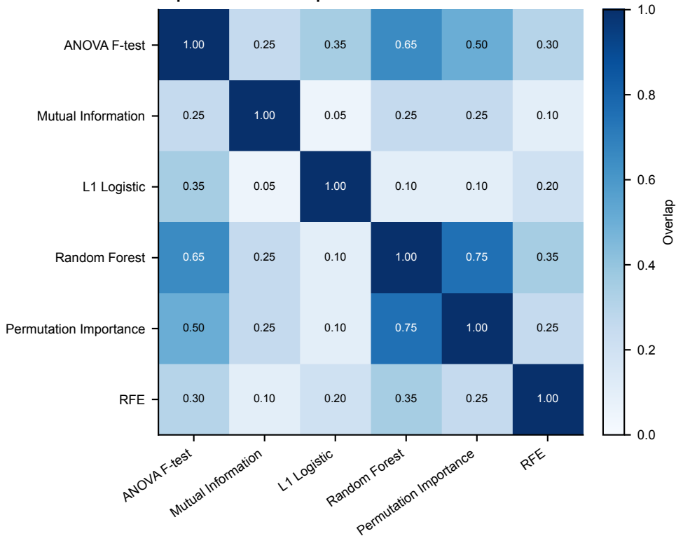
Top-20 feature overlap across selectors
