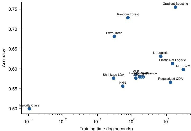
Accuracy vs training time
