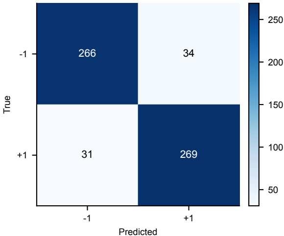
Confusion matrix: Best FS: Random Forest + Random Forest (k=20)
