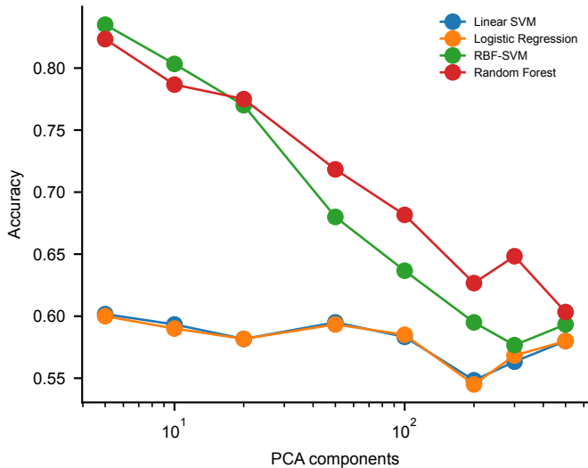
a PCA dimension vs accuracy
