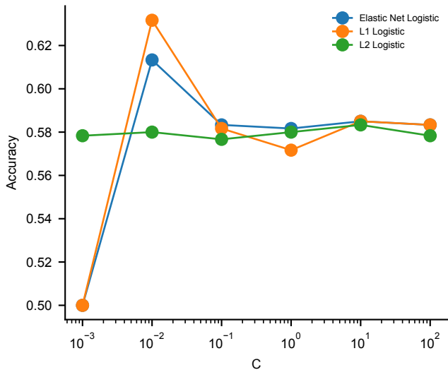
a Regularization strength vs accuracy
