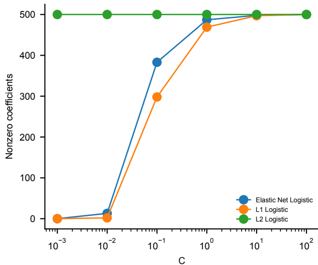
b Regularization strength vs sparsity
