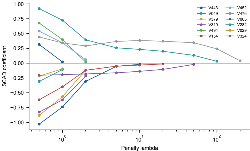
Largest SCAD coefficients across penalty strengths
