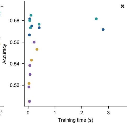
Accuracy-time trade-off
