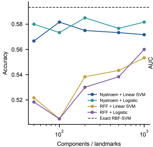
Approximation dimension
