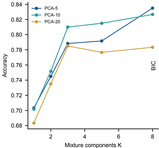
Best EM-GMM accuracy over covariance types
