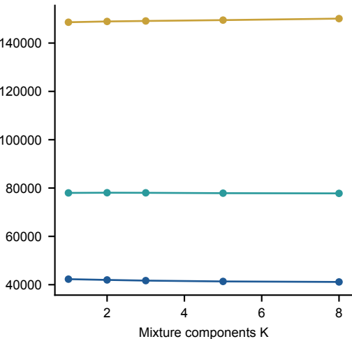
Minimum BIC over covariance types
