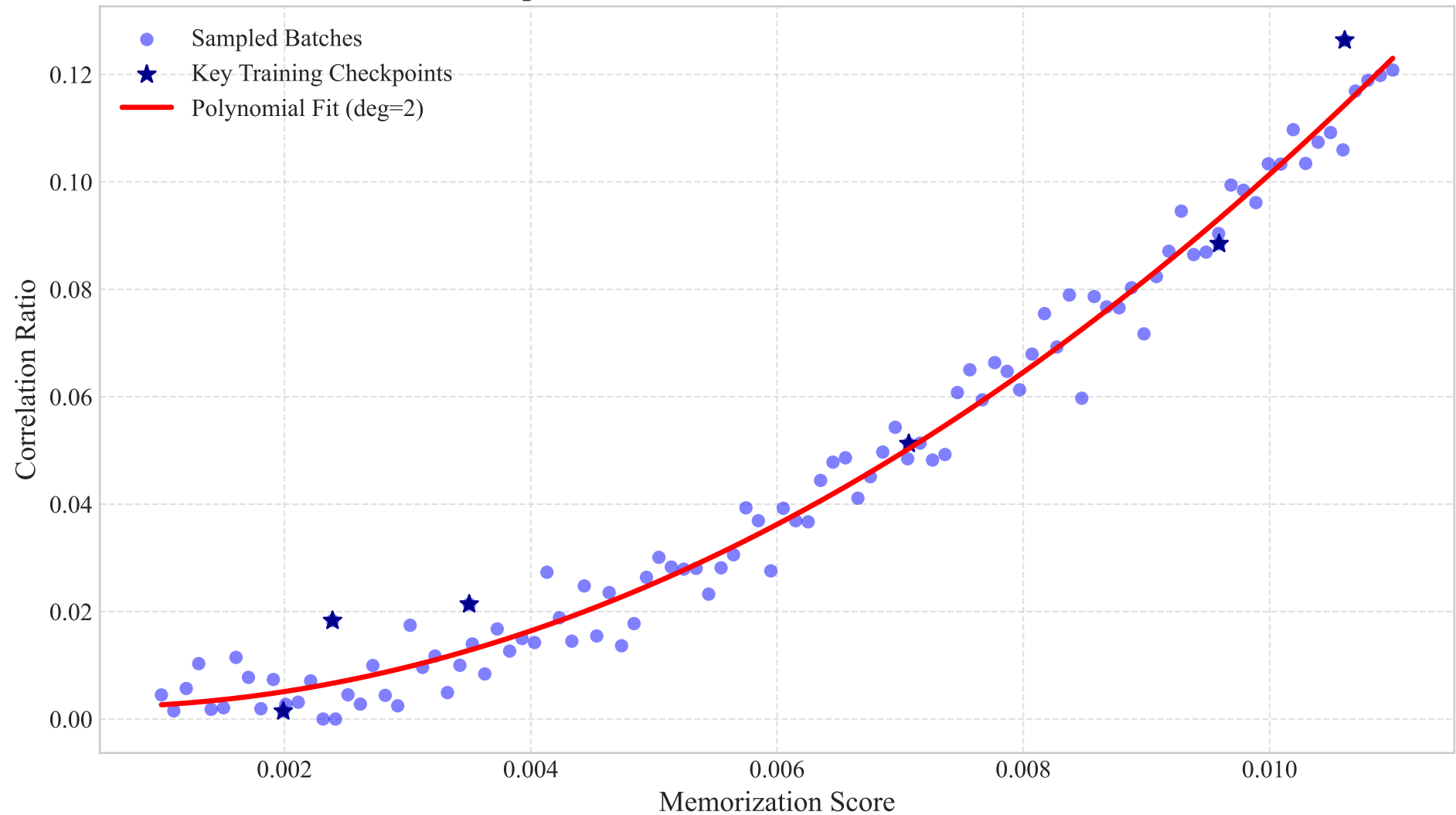
Relationship between Memorization and Correlation Ratio
