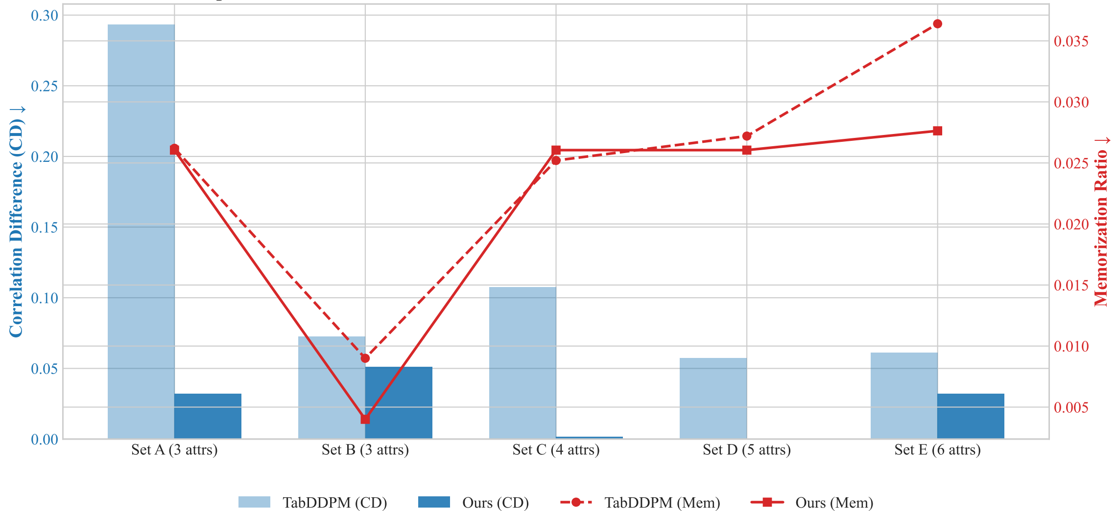
Impact of Attribute Combinations on Correlation Preservation and Memorization
