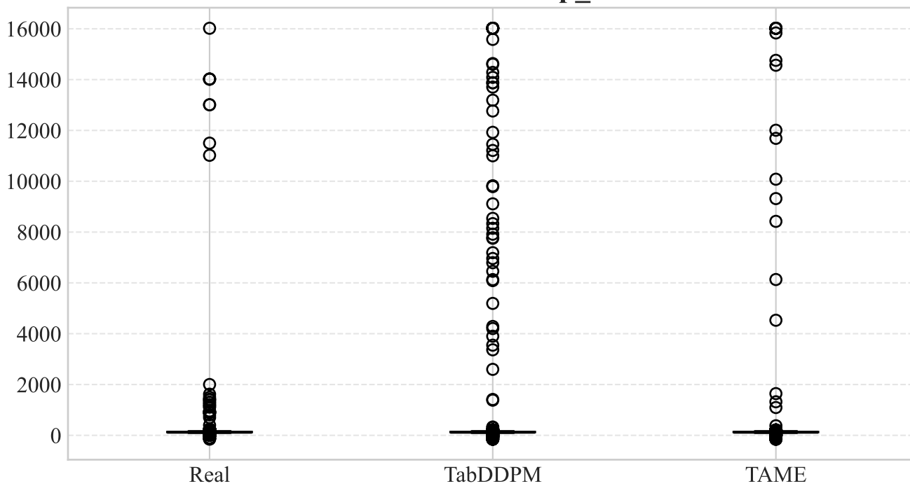
Distribution: ap_hi
