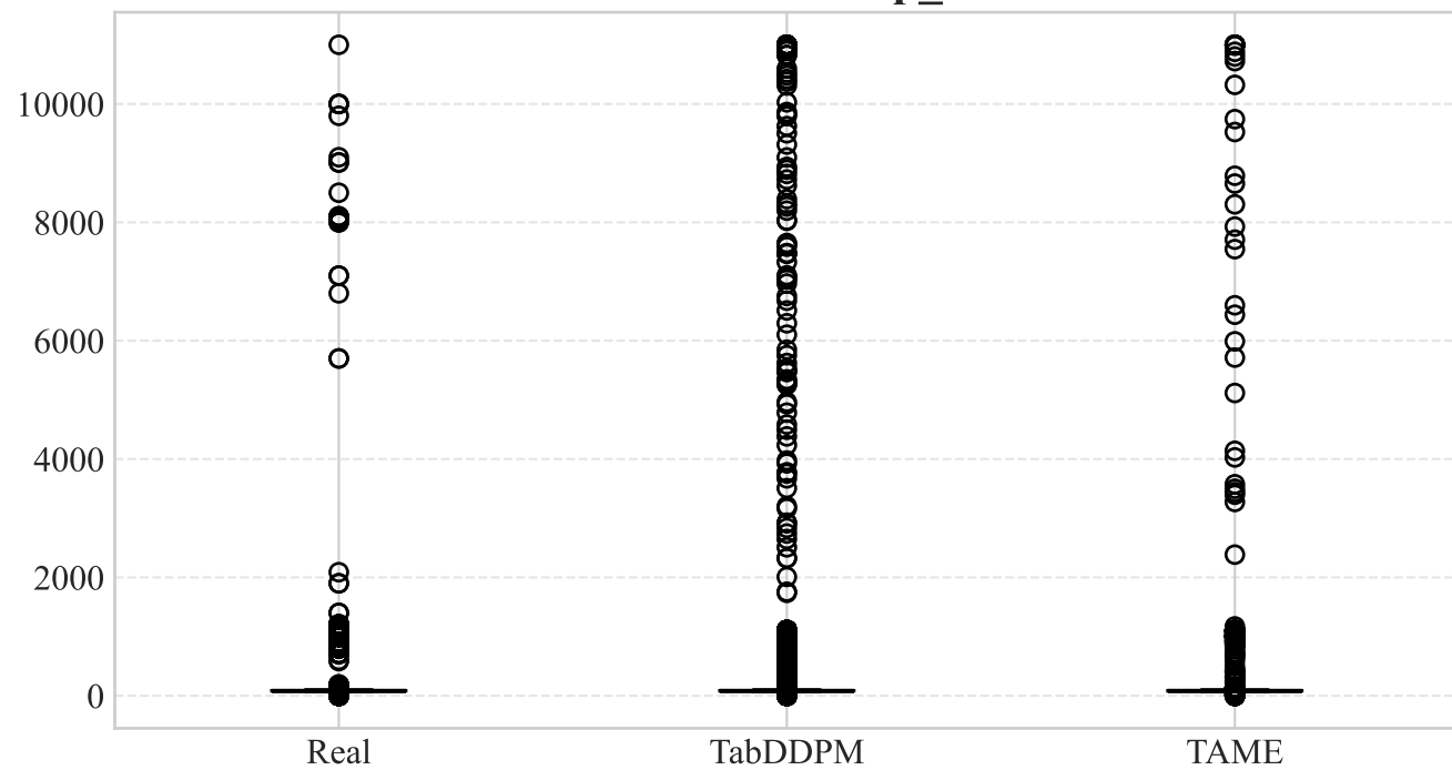
Distribution: ap_lo
