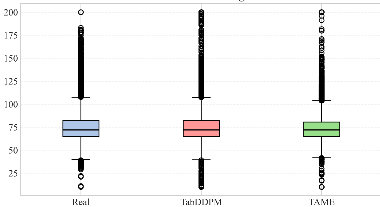
Distribution: ap_lo
