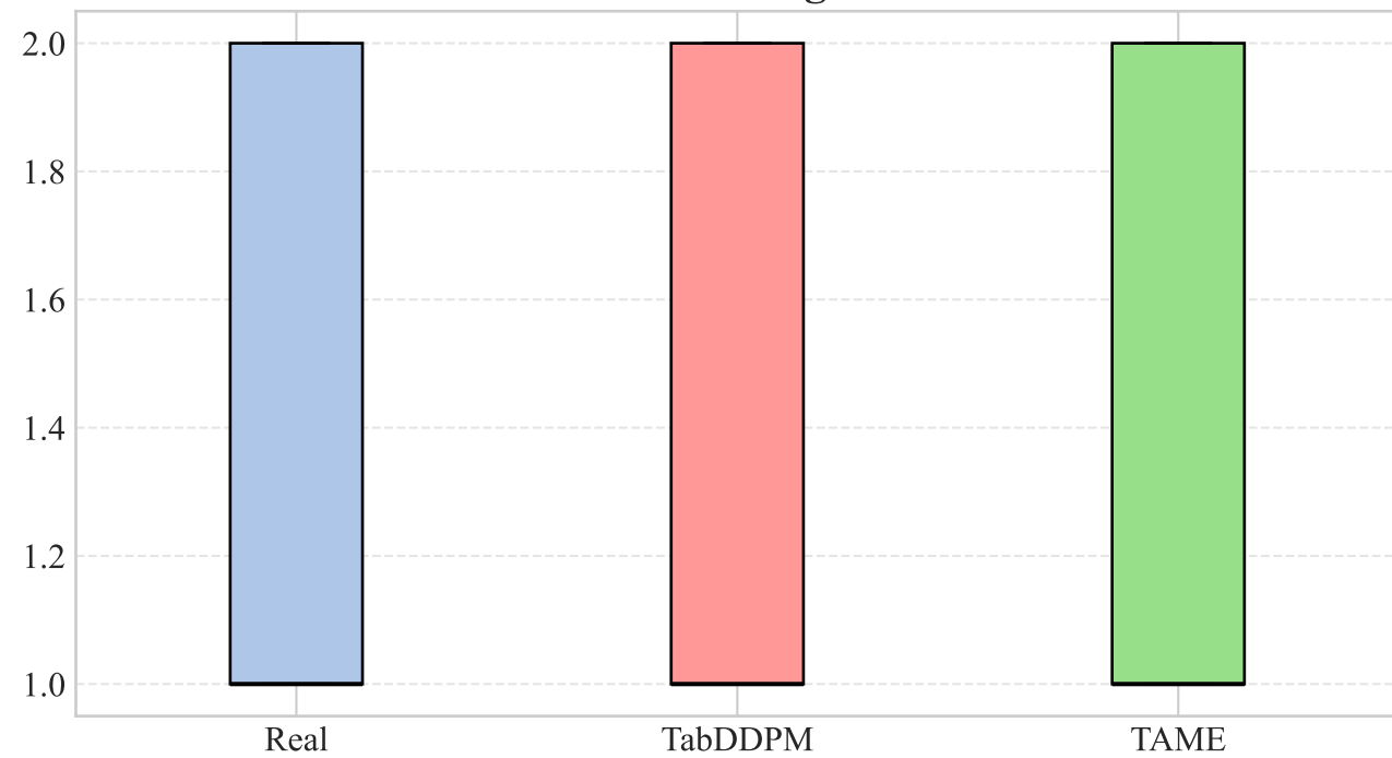
Distribution: weight
