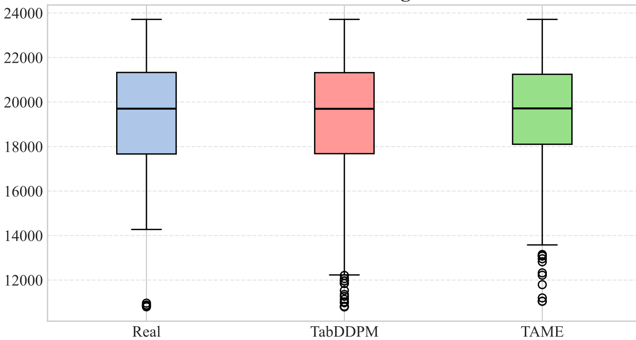
Distribution: height
