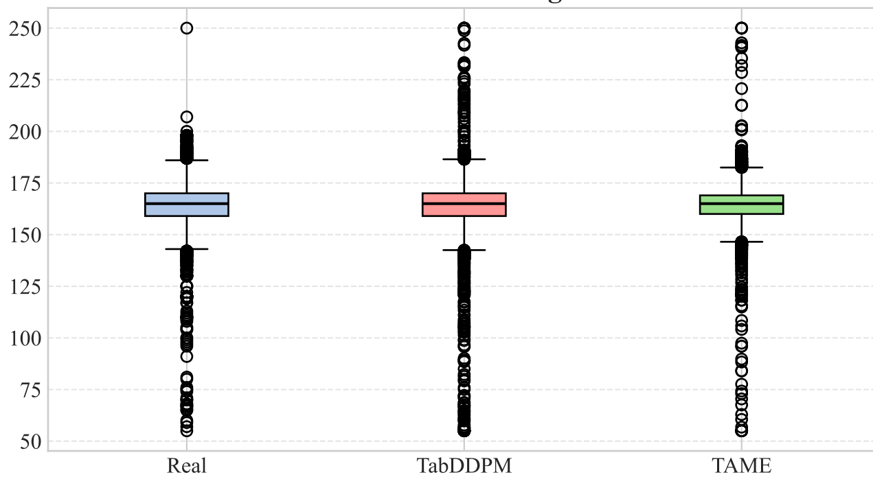
Distribution: ap_hi
