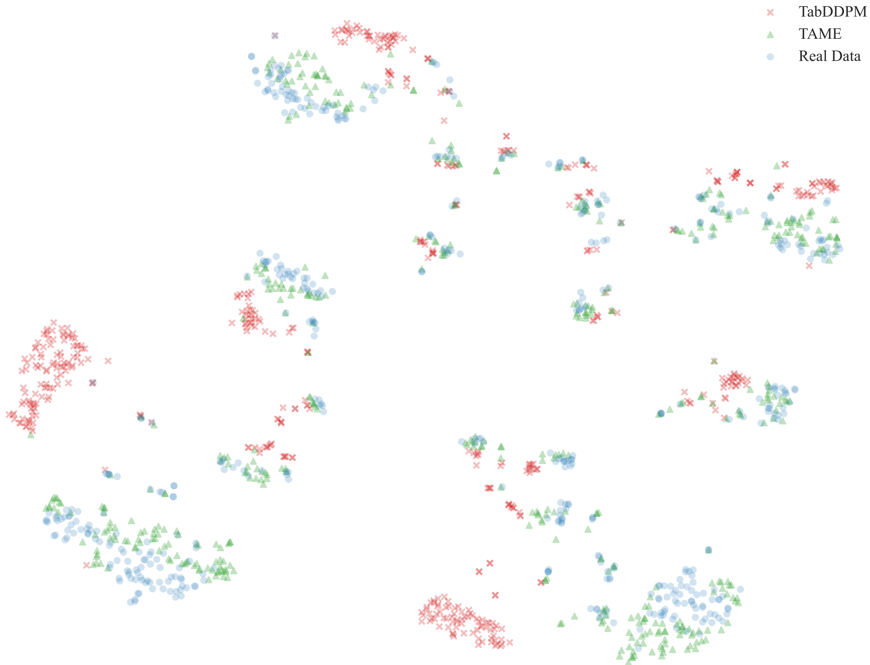
t-SNE Visualization of Data Manifold - cardio
