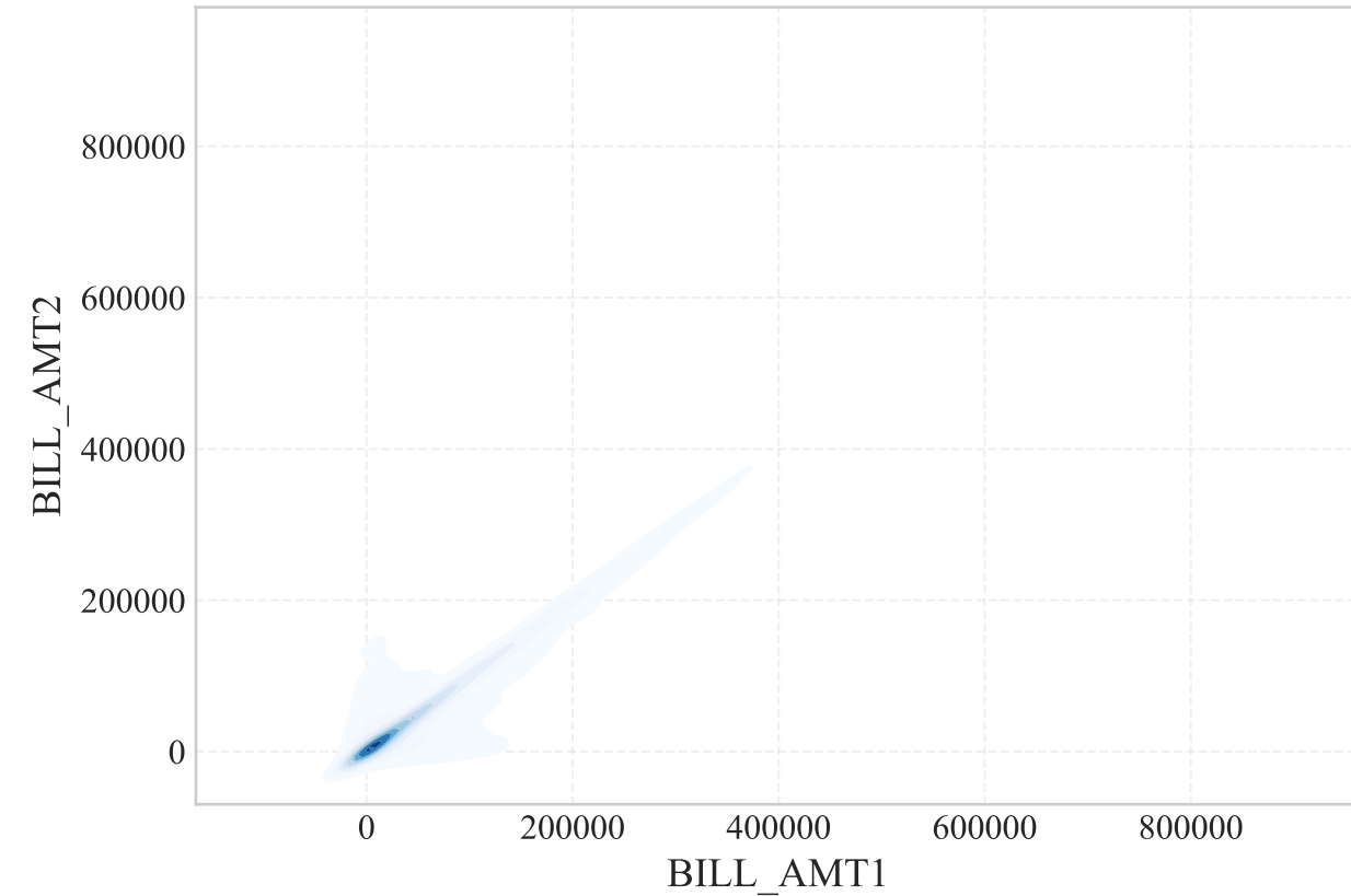
Real Data (BILL_AMT1 vs BILL_AMT2)
