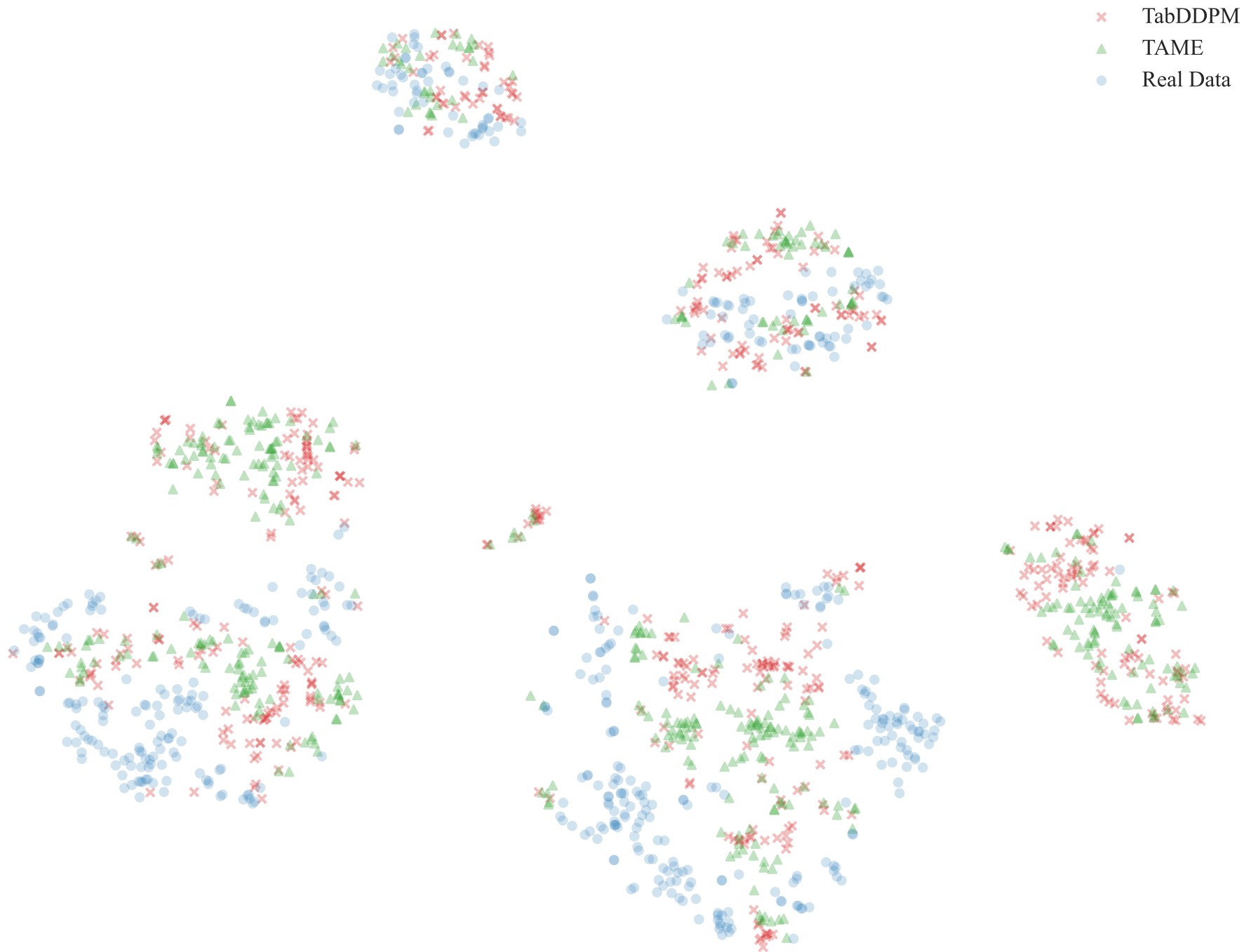
t-SNE Visualization of Data Manifold - default
