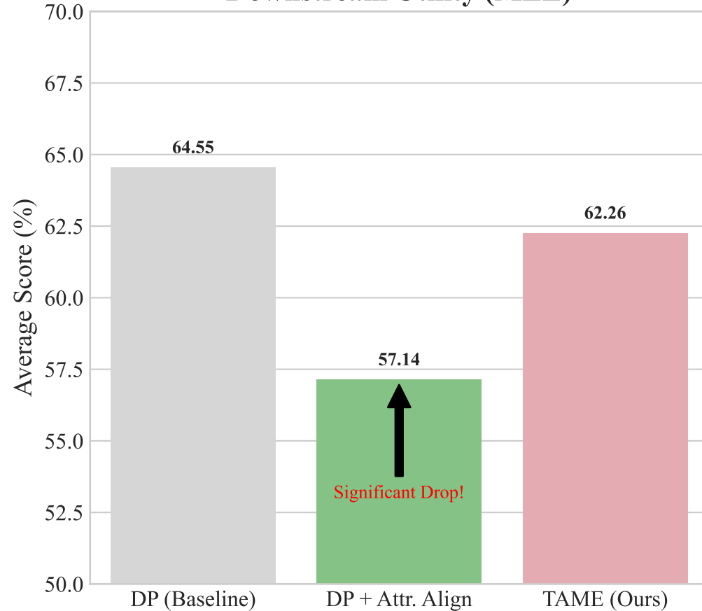
Downstream Utility (MLE)
