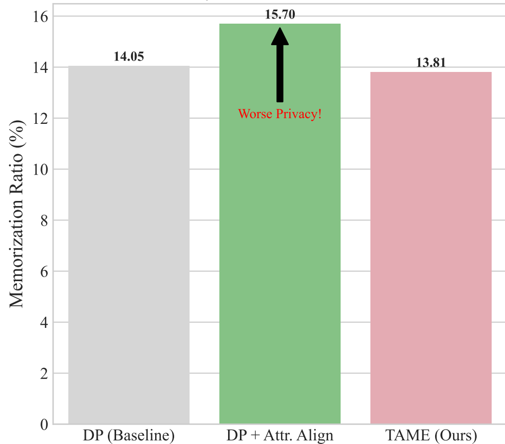
Privacy Risk (Memorization)
