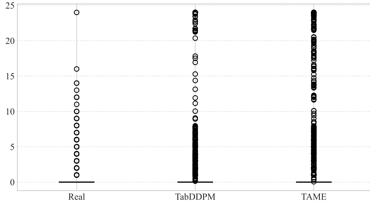
Distribution: ProductRelated
