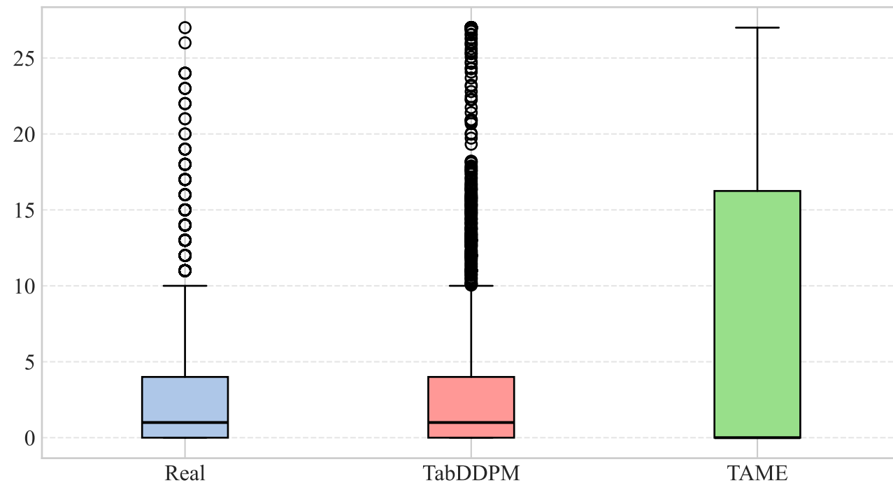
Distribution: Informational
