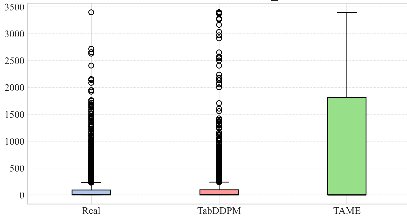
Distribution: Informational_Duration
