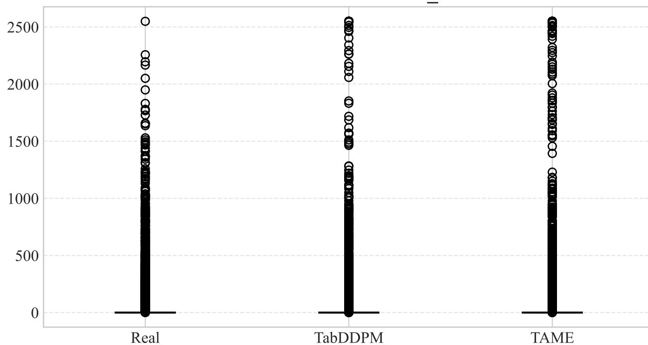
Distribution: ProductRelated_Duration
