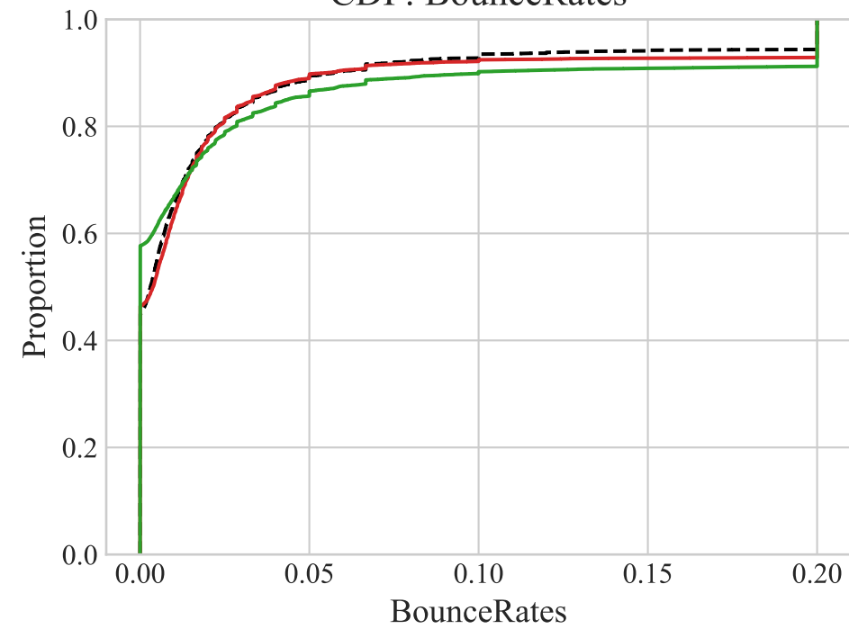
CDF: BounceRates
