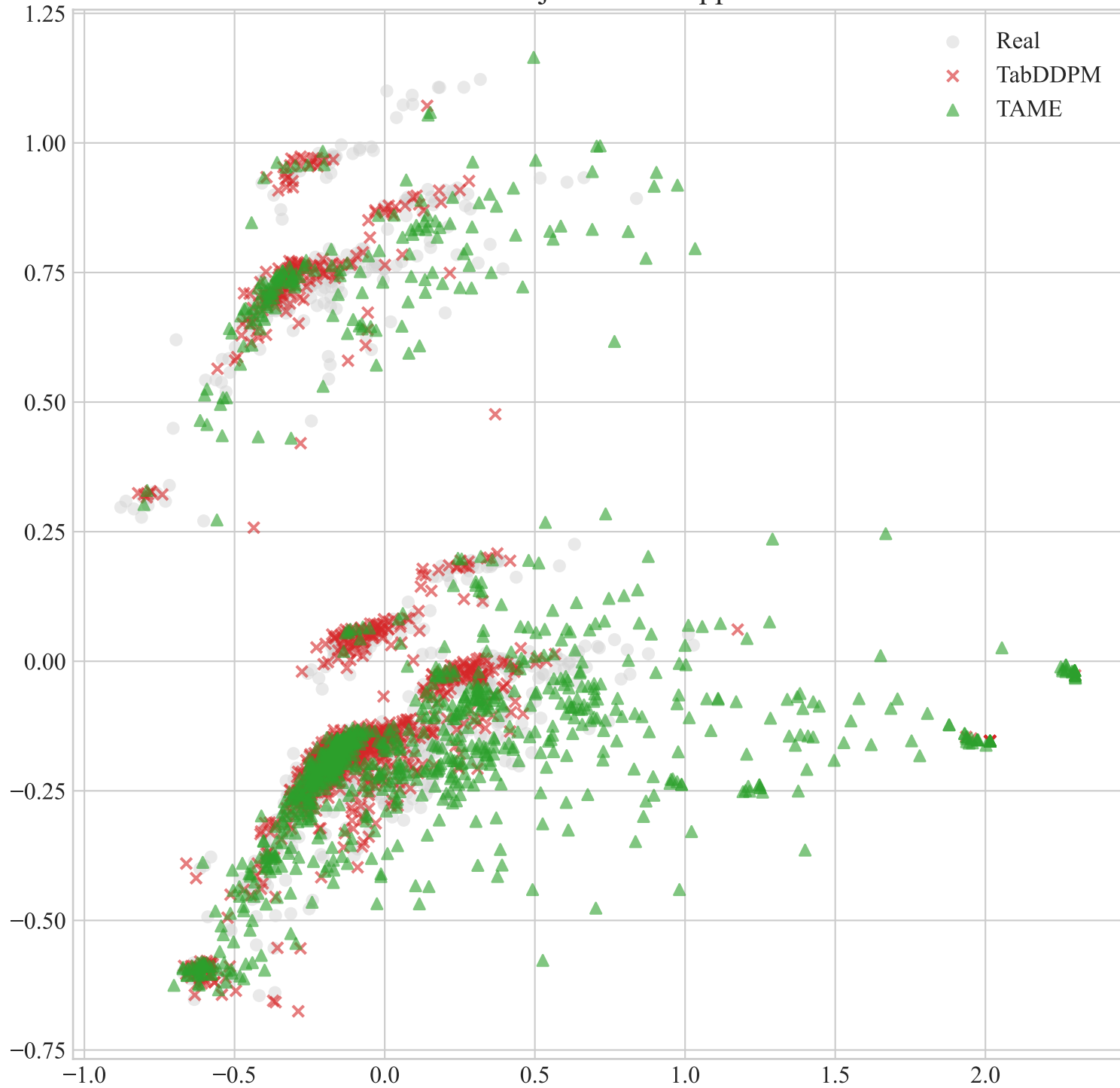
PCA Projection - shoppers
