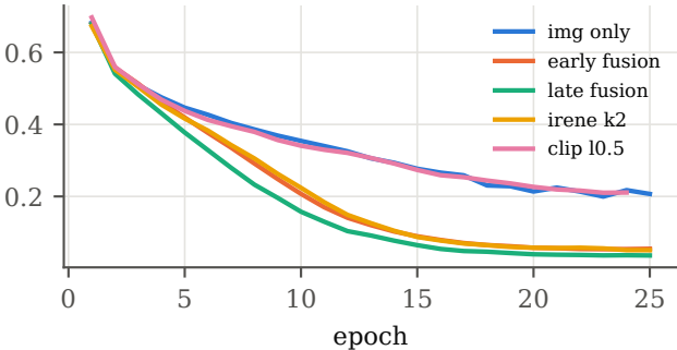
(a) Training BCE
