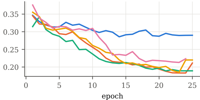
(b) Validation BCE (inner split)
