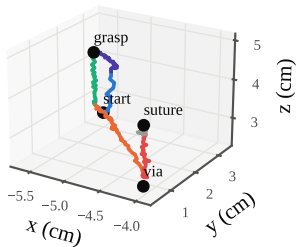
(a) Tool path in the ECM frame
