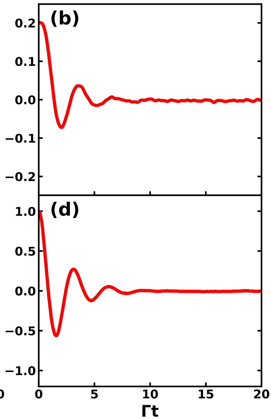
SBM #4
