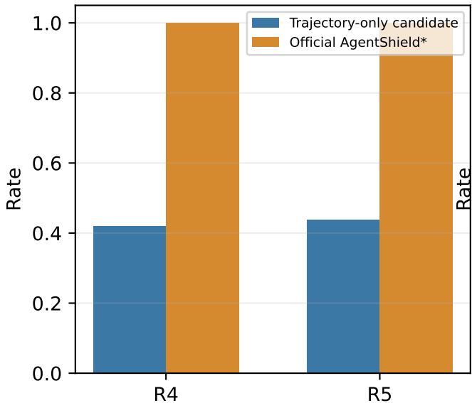
Successful-attack recall
