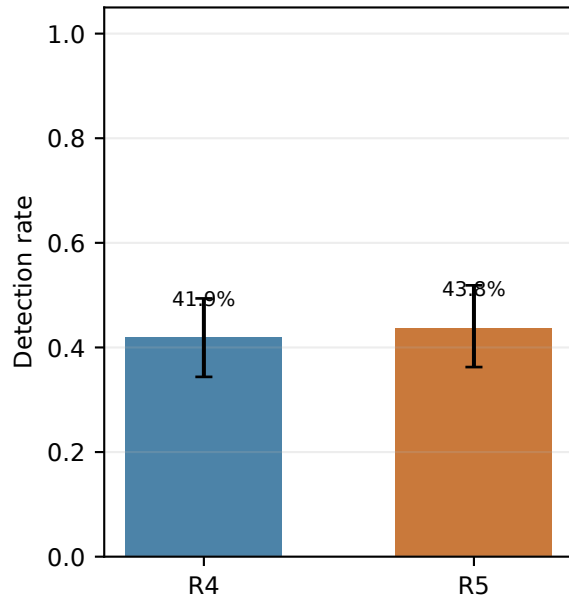
Successful attacks
