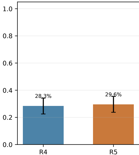
All attempts
