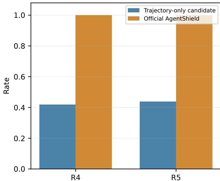
Successful-attack recall
