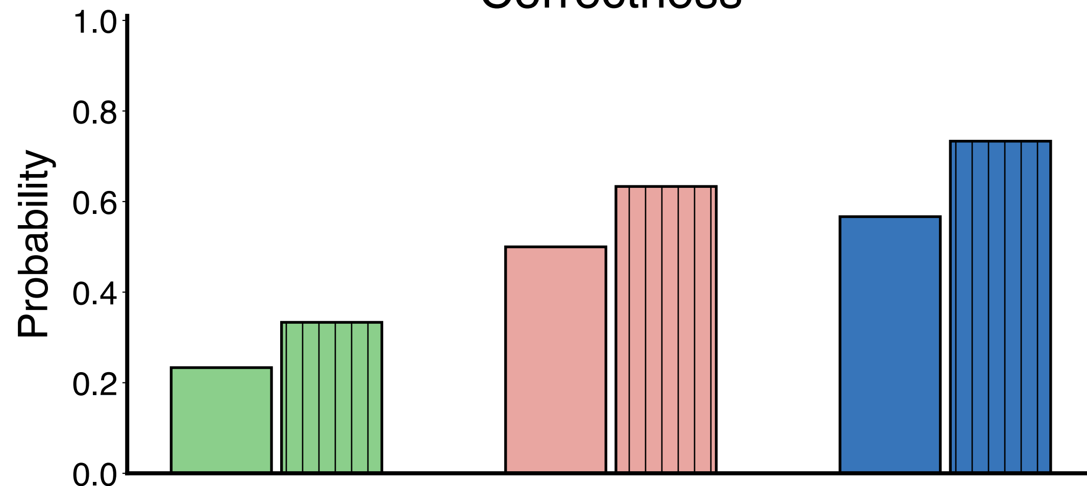
Correctness
