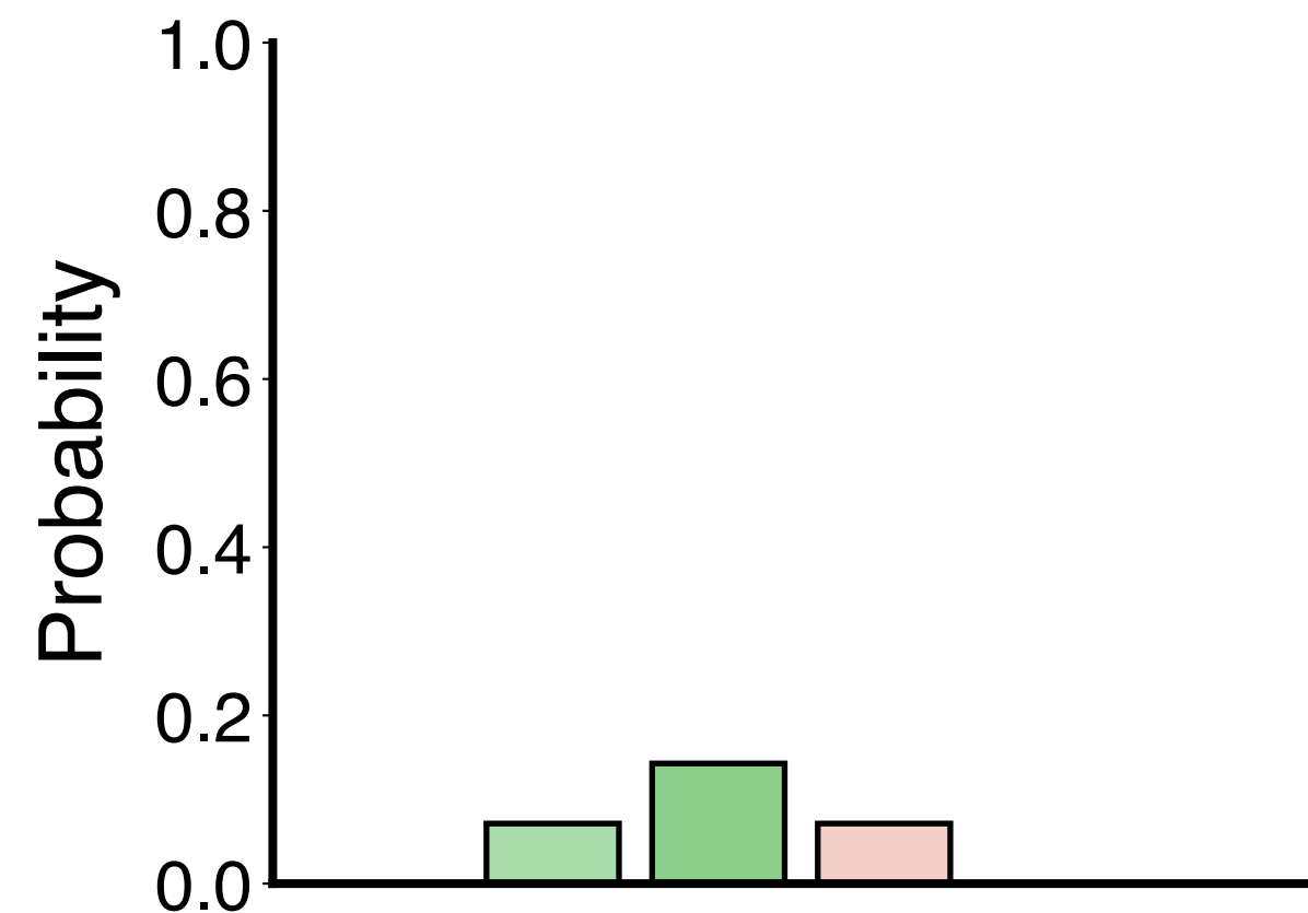
Justified denial ↑
