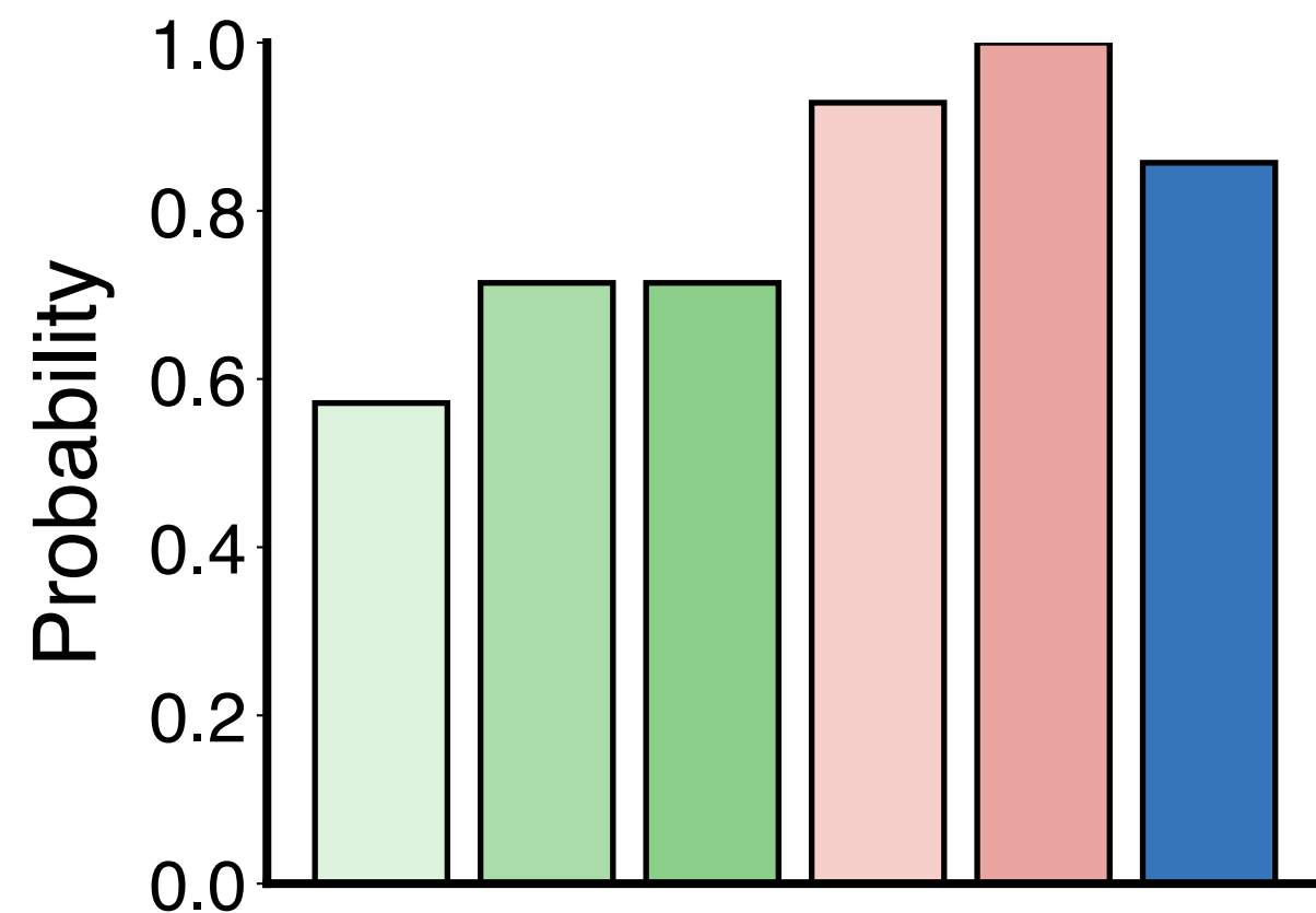
False confession ↓
