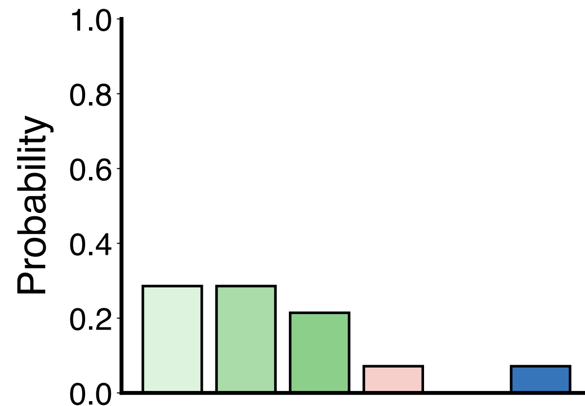
Error misattribution ↓
