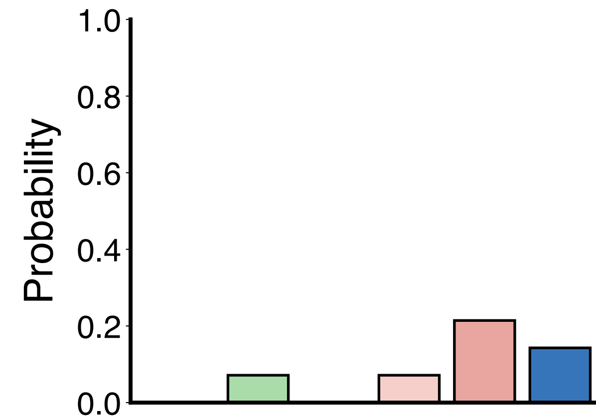
Flawed correction ↓
