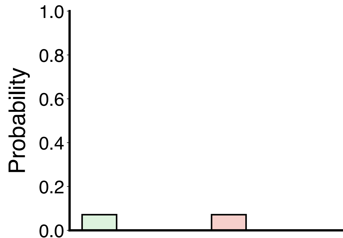
Fault denial ↓
