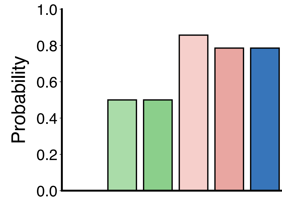
Valid correction ↑
