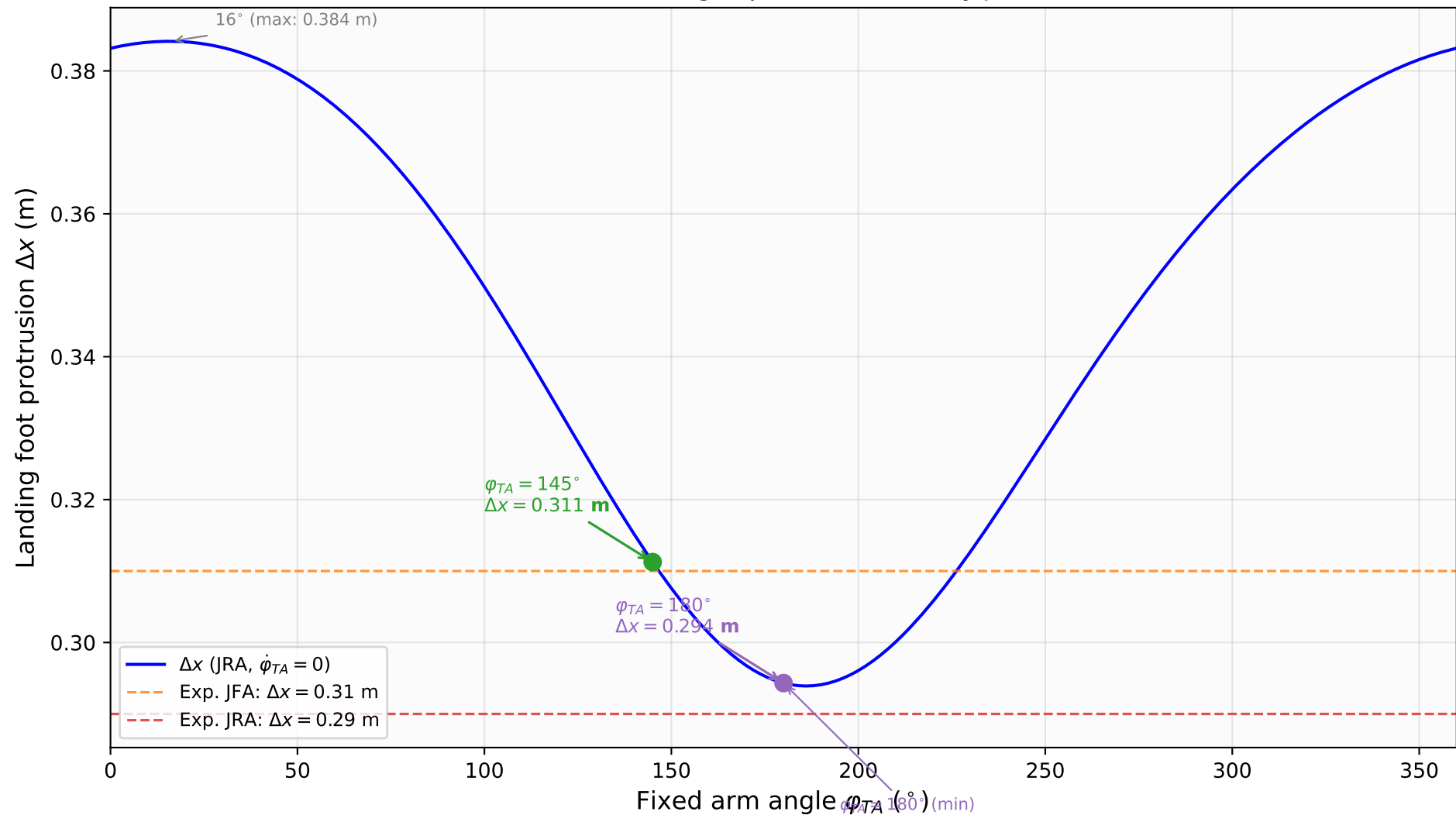
\Delta x vs. static arm angle \phi_{TA} in three-body JRA ( L_0 = 0 )
