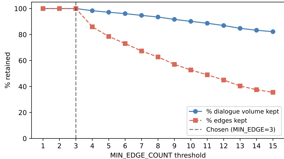
Volume vs edges retained at each threshold
