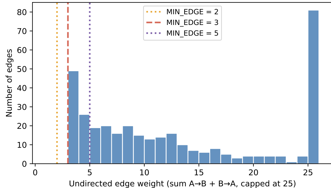
Distribution of undirected edge weights (production pipeline, all 17 films)
