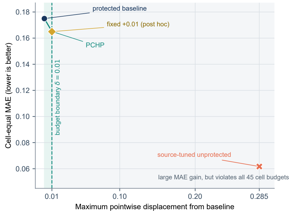
B Harm-control--accuracy trade-off
