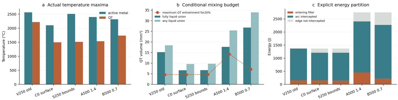
Ni99 first short track · source model and deposition geometry decision
