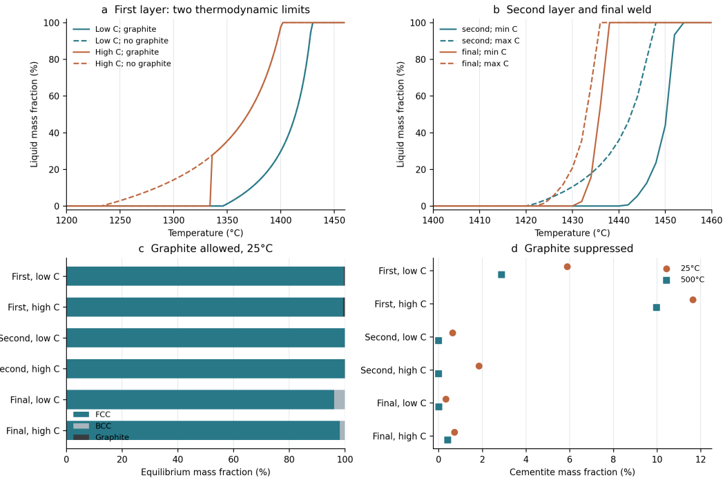
Fe-Ni-C layer composition corners · CALPHAD calculation
