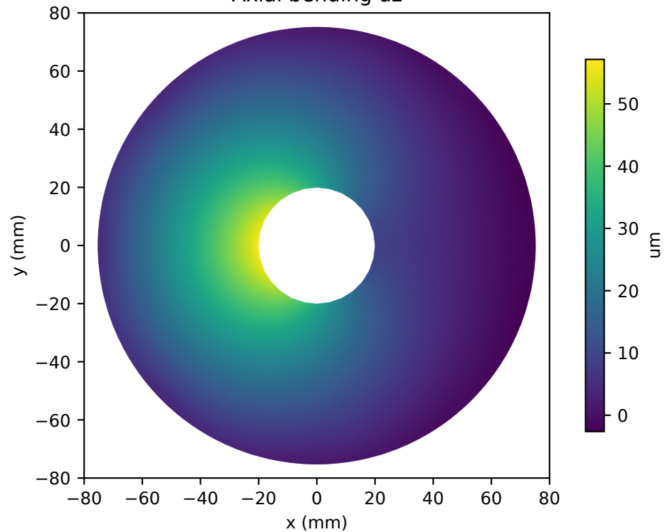
Axial bending u_z
