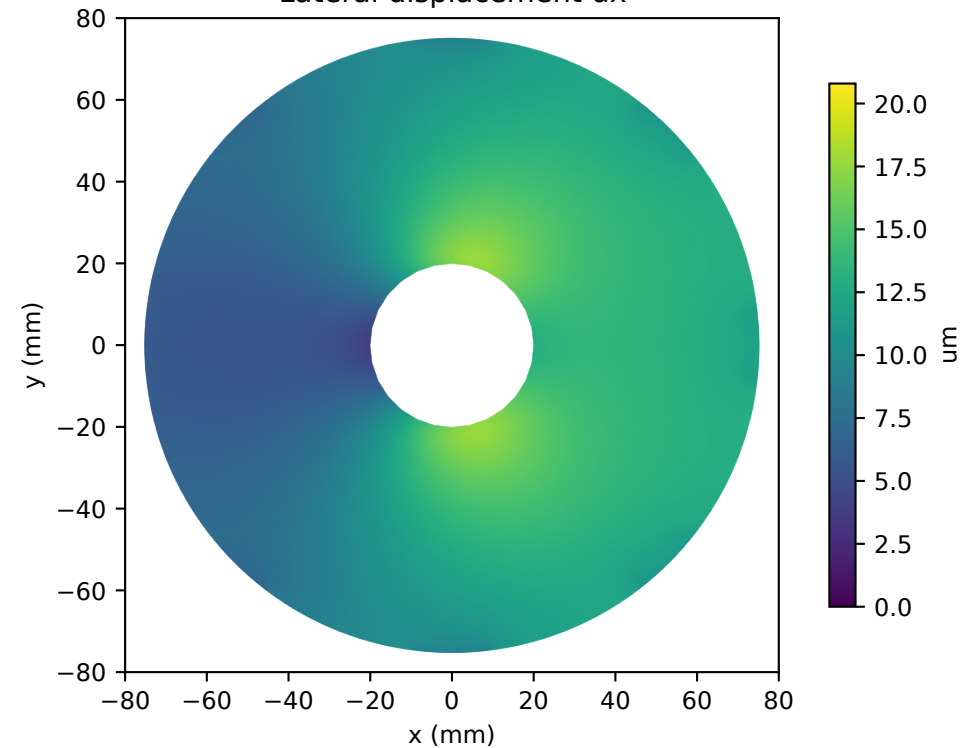
Lateral displacement u_x
