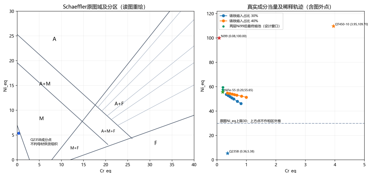
Figure 1. Schaeffler original diagram and dilution trajectory
