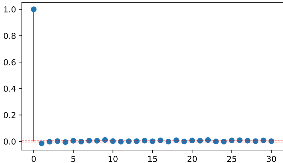
MOUF: Gaussianized PIT ACF
