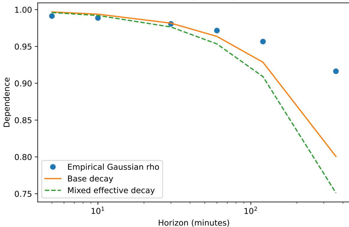
Multi-horizon temporal dependence
