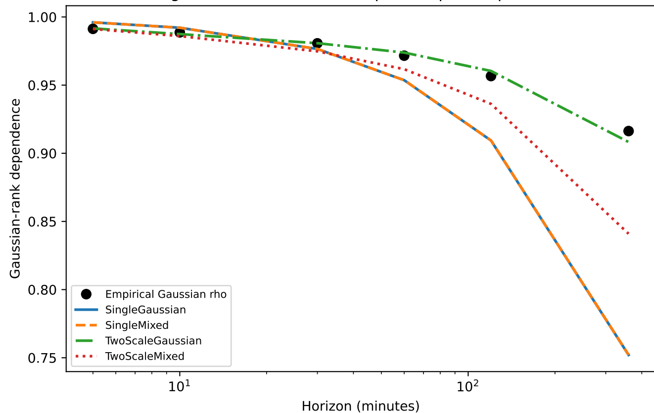
Single- versus two-scale temporal copula dependence
