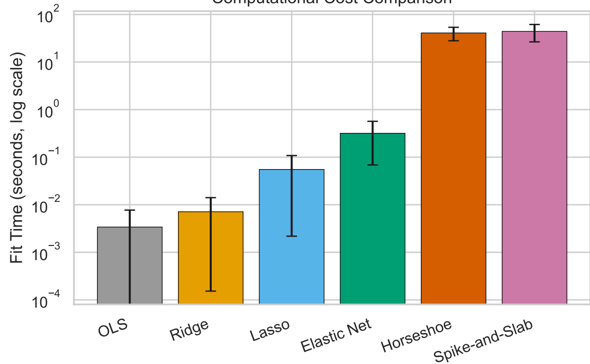
Computational Cost Comparison
