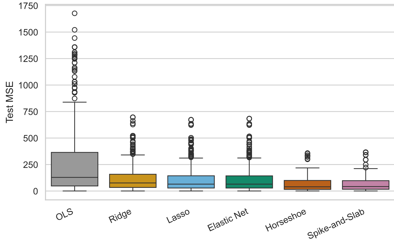
Test MSE Distribution Across Random Seeds
