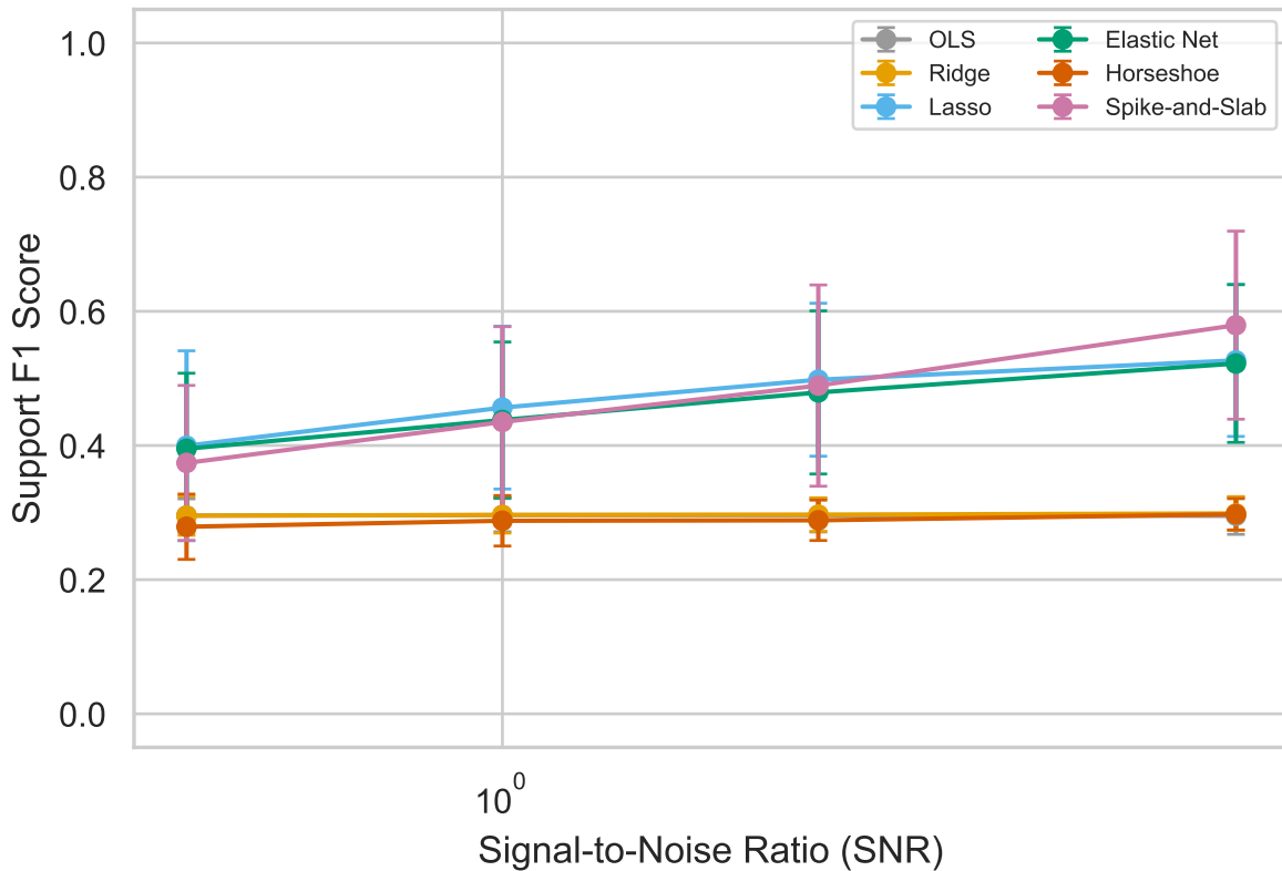
Variable Selection Performance vs Signal Strength
