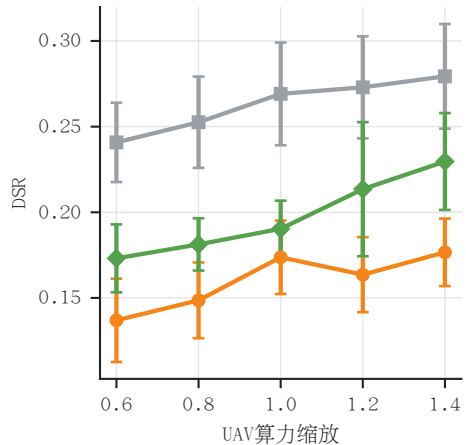
DSR
