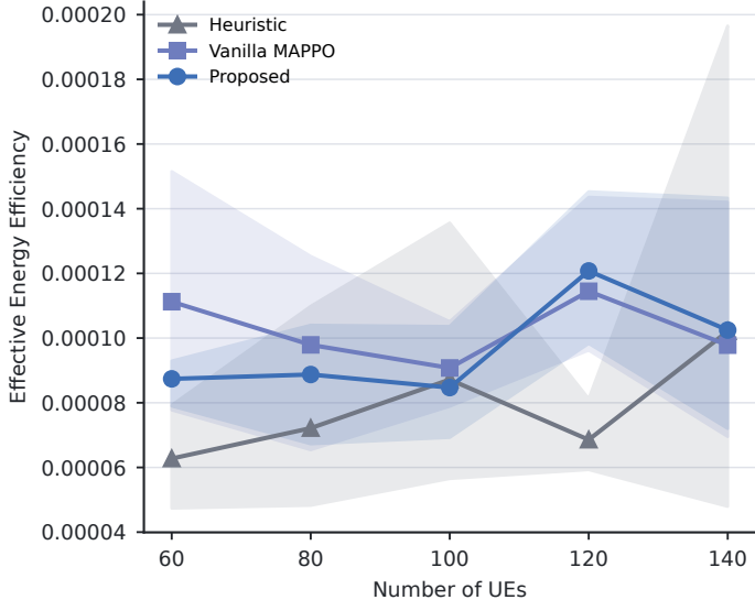
Effective energy efficiency
