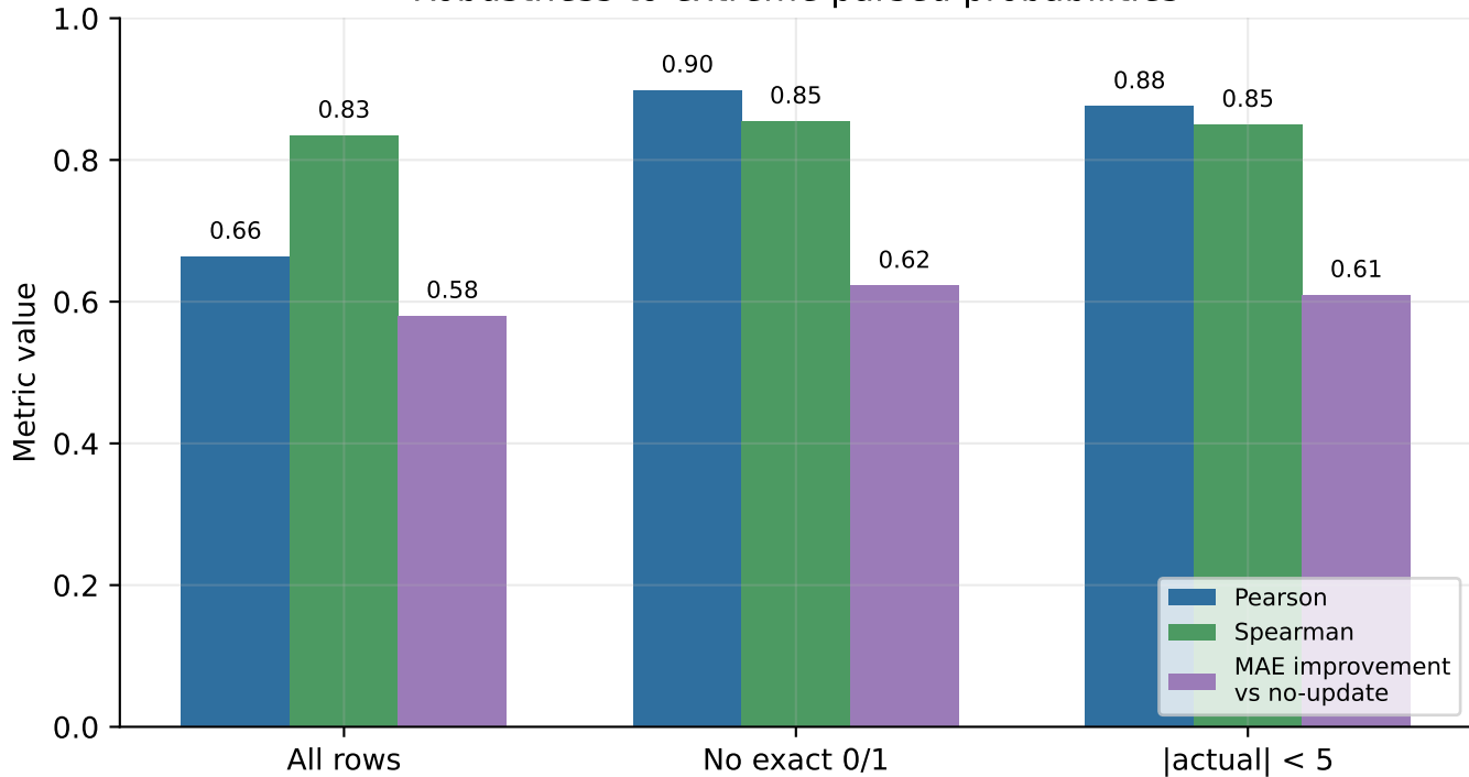
Robustness to extreme parsed probabilities
