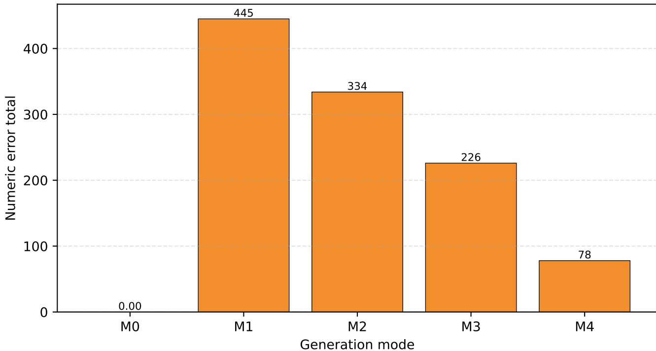
Numeric Errors by Mode (91 days)
