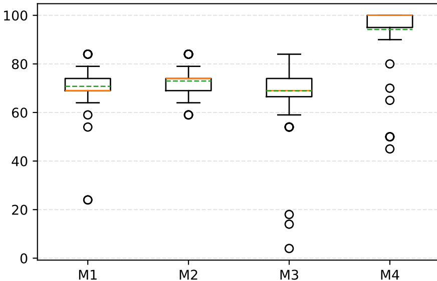
Unsupported claims
