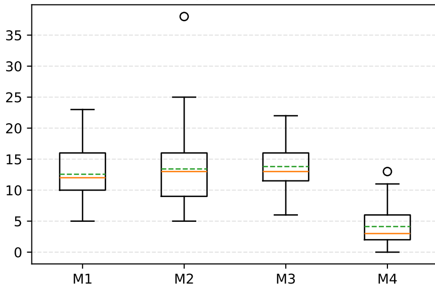
Unsupported claims
