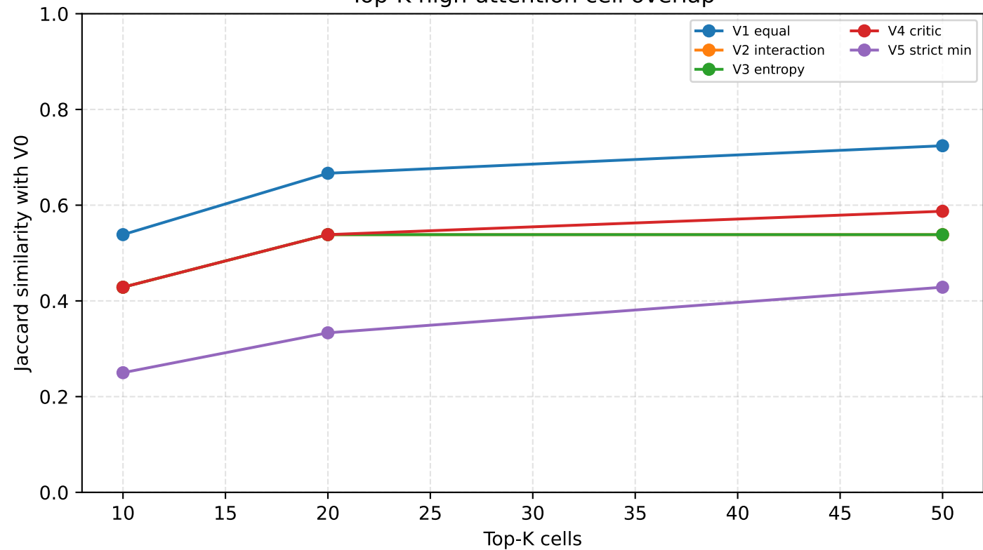
Top-K high-attention cell overlap
