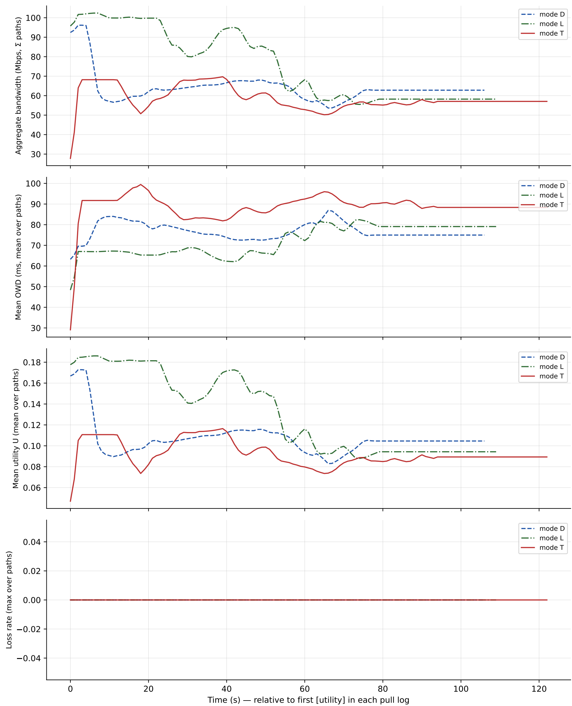
MPQUIC utility modes: T (throughput) vs D (delay) vs L (loss)
