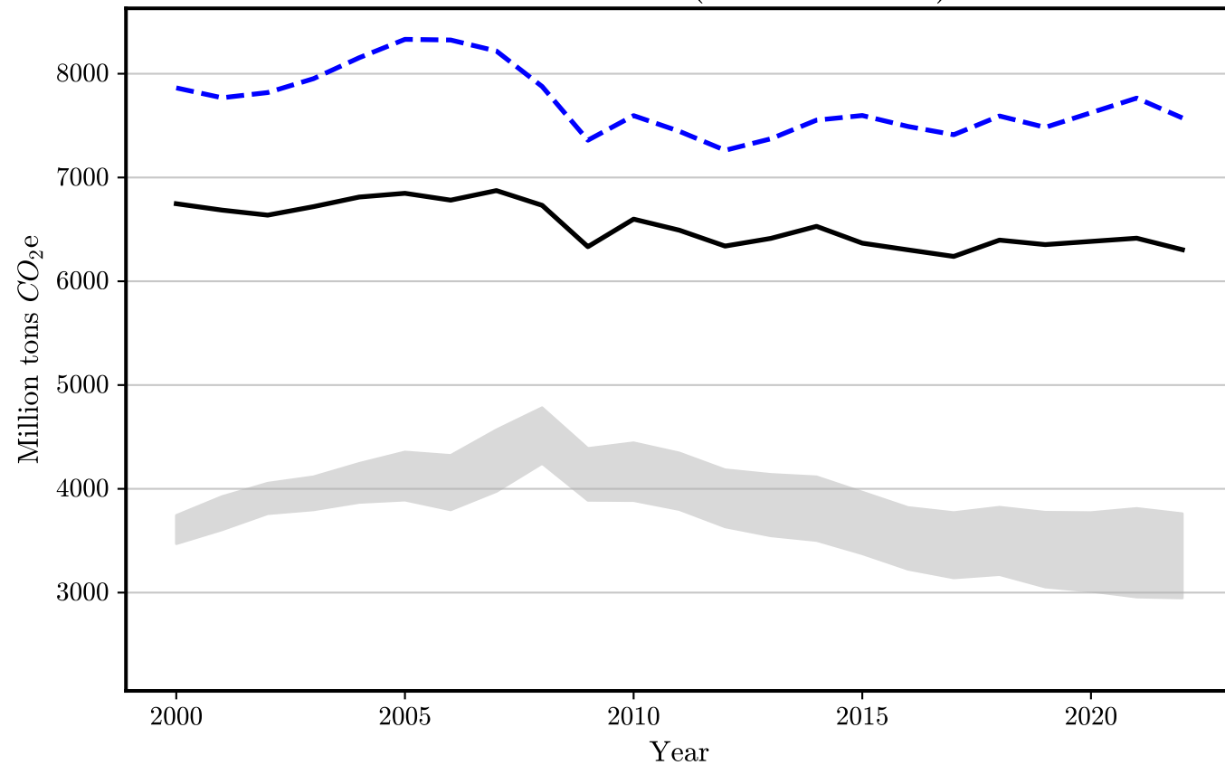
GHG Emissions (United States)
