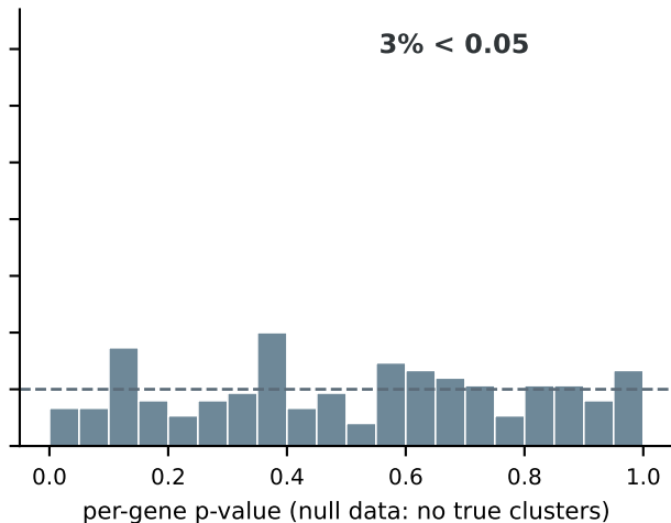
Count splitting (cluster on fold 1, test on fold 2)
