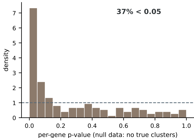
Double dipping (cluster and test on X, same test)
