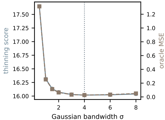
both criteria minimised at the same \sigma
